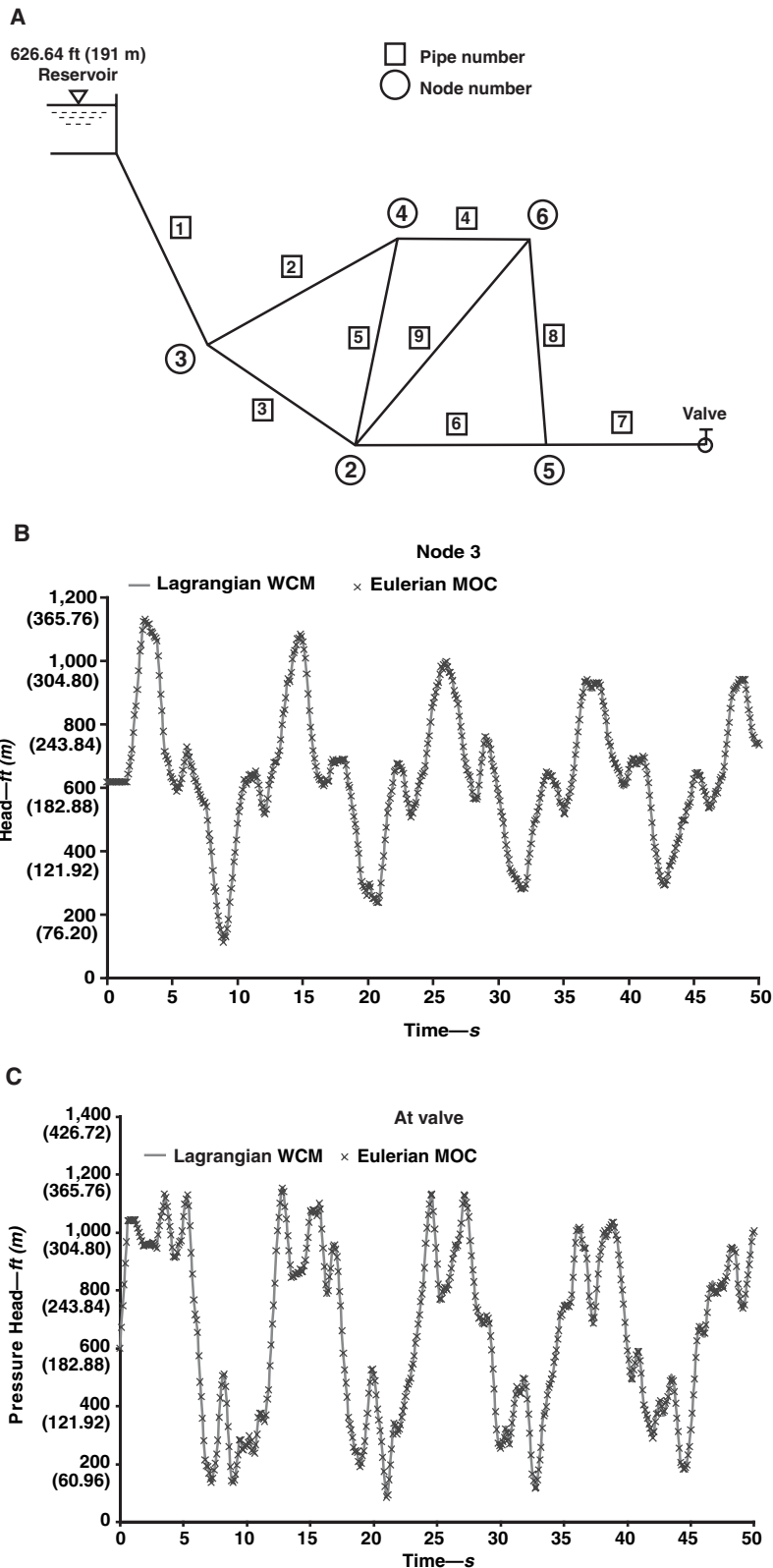
FIGURE 3 Pipe network schematic and pressure head at node 3 and valve for Example 2
