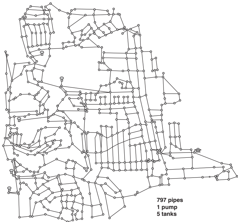
FIGURE 7 Pipe network schematic for Example 4
