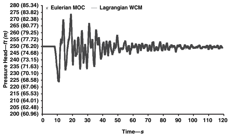
FIGURE 9 Comparison of results at node 3066 for Example 4
