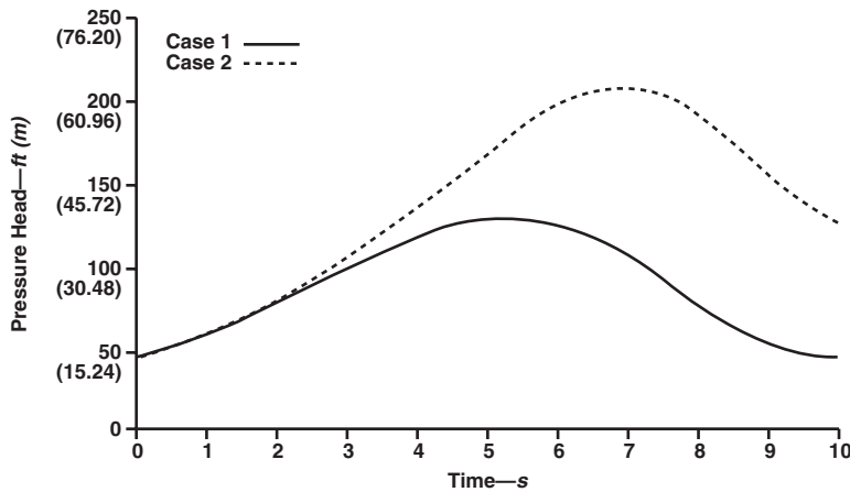
FIGURE 2 Pressure head variations at valve
